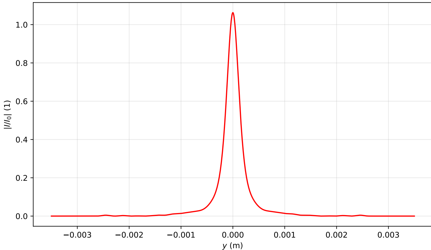
Intensity profile I(x = 0, y, z = 3.025)/I_0 , P_{in}=4.0P_{cr} , artificial time
